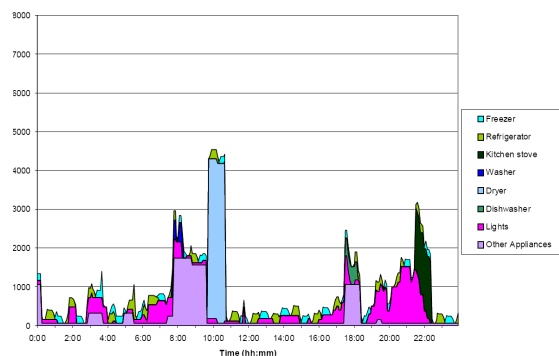
Typical daily load distribution of a household
