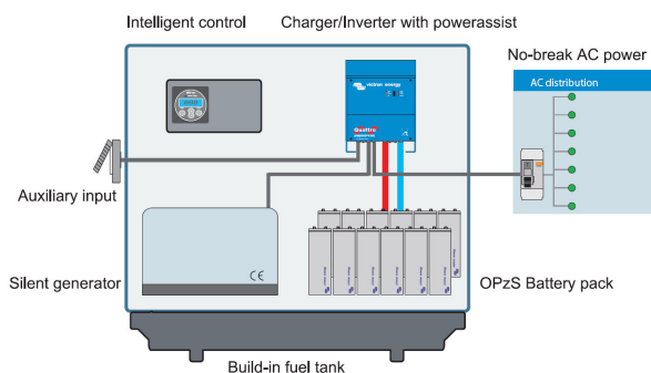
Block diagram
